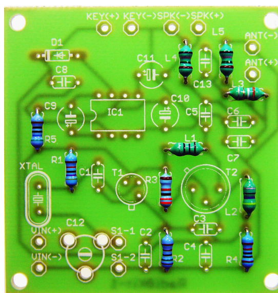
The board after soldering the inductors.
